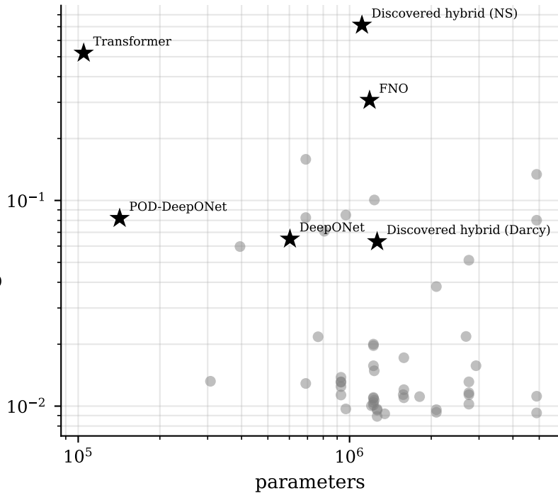
Darcy 2D
