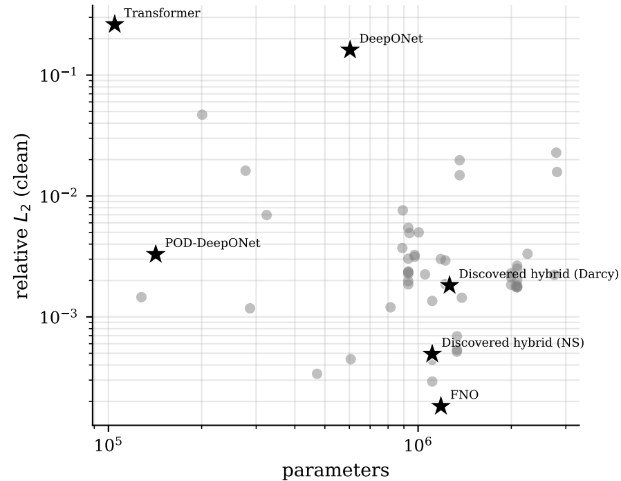
Navier-Stokes 2D
