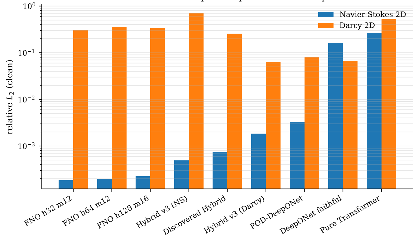
No universal winner: optimal operator is PDE-dependent
