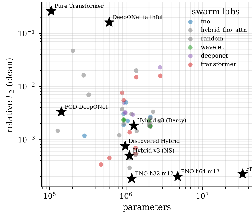
Navier-Stokes 2D
