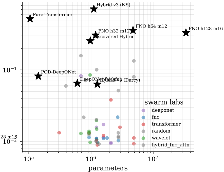
Darcy 2D
