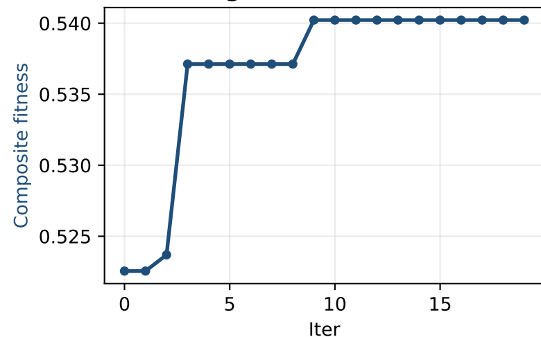
Burgers (1D) - fitness
