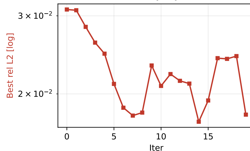
Linear Advection (1D) - best rel L2
