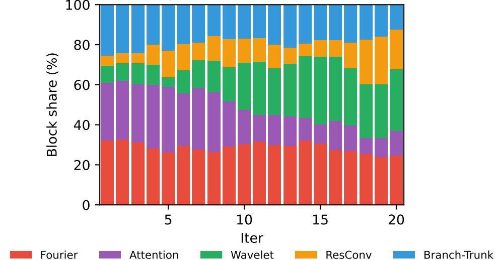
Piecewise Regression (1D) - block evolution
