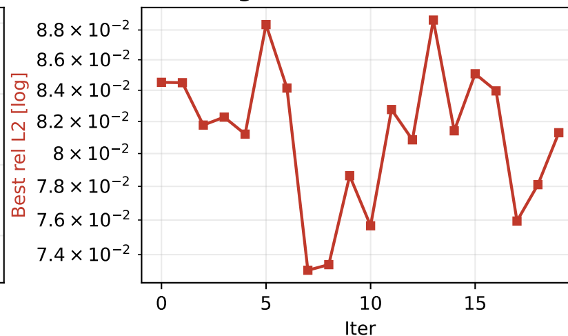
Burgers (1D) - best rel L2
