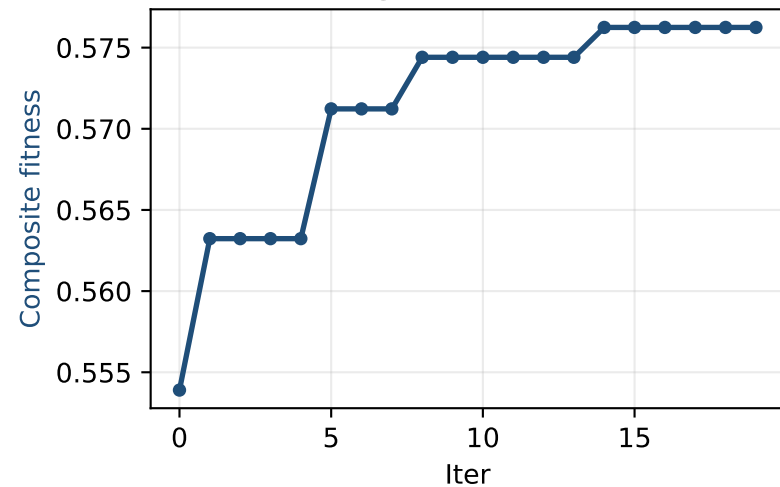
Piecewise Regression (1D) - fitness
