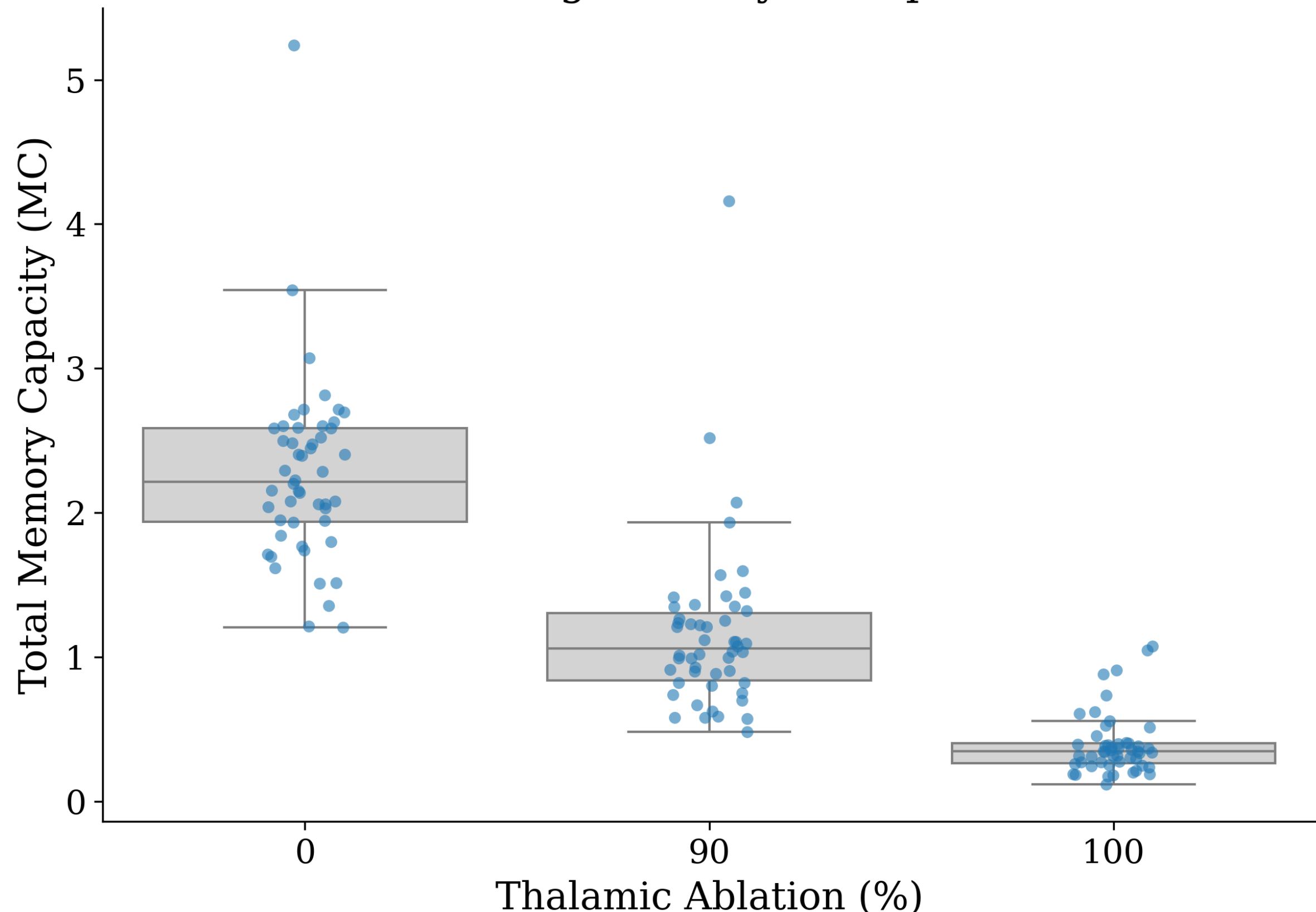
Figure: Temporal Integration. The baseline M_{cc} maintains temporal memory, while complete
