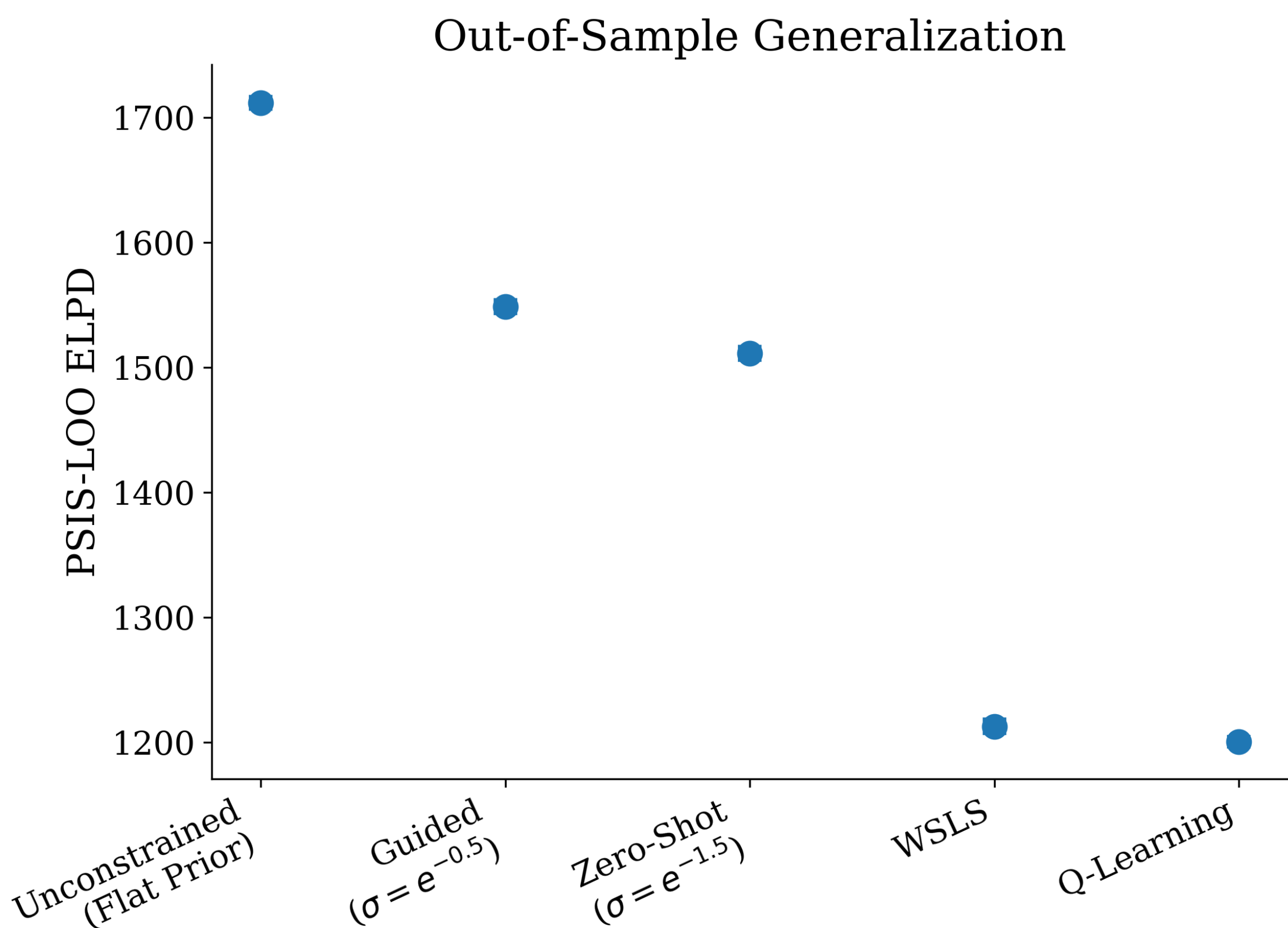
Figure: Zero-Shot Transfer. The distilled physiological model predicts raw behavior significantly better than natively optimized heuristics.
