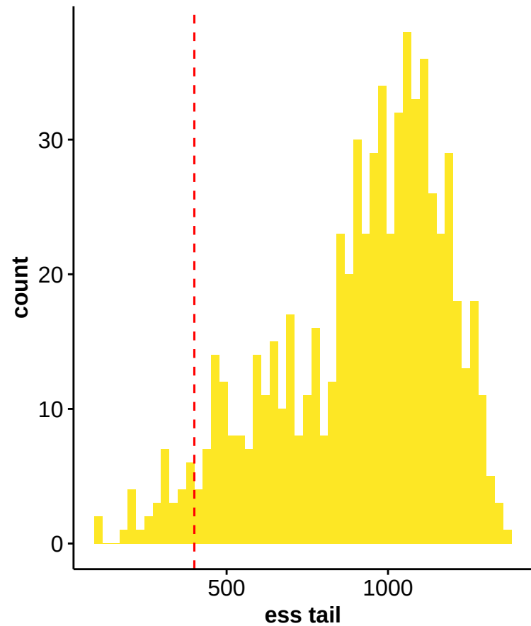
ess tail distribution
