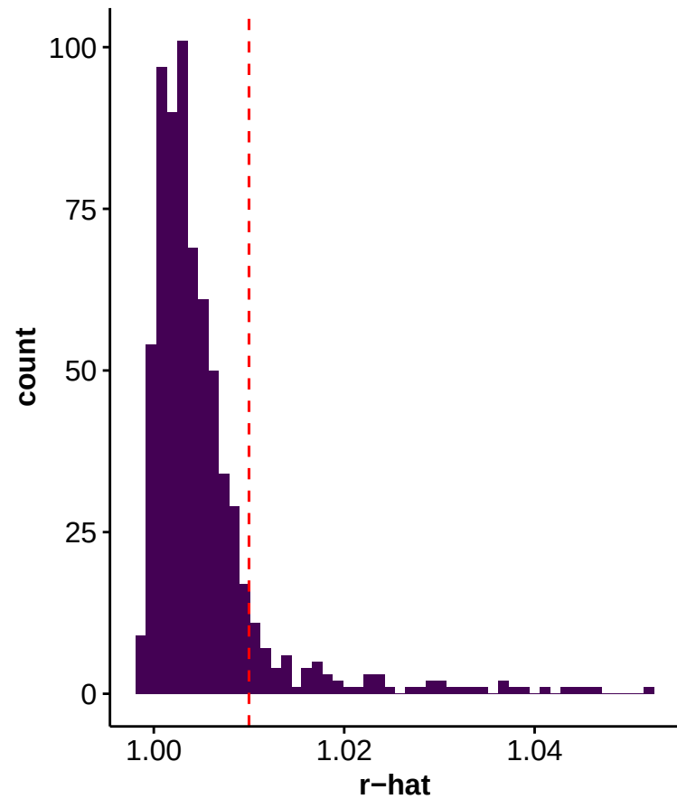
r-hat distribution (full gating)
