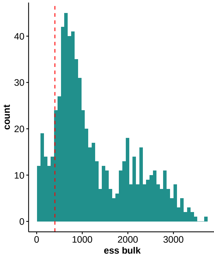
ess bulk distribution
