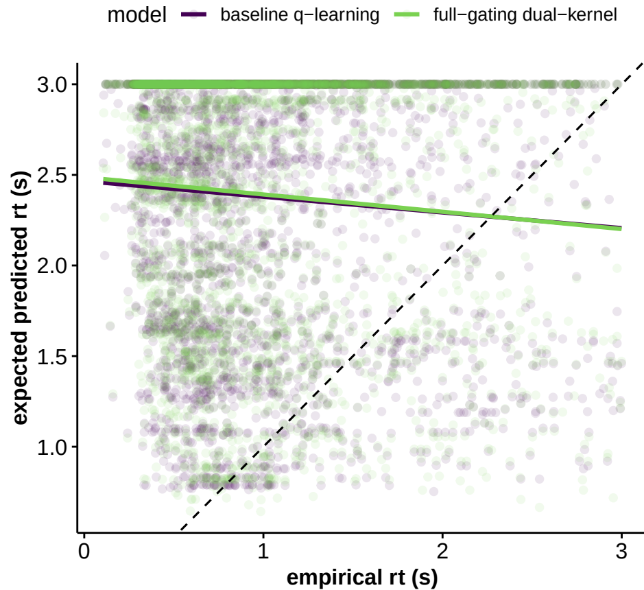
ppc: reaction times
