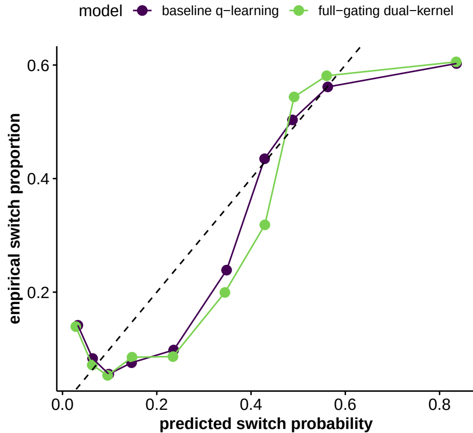
ppc: switch proportions
