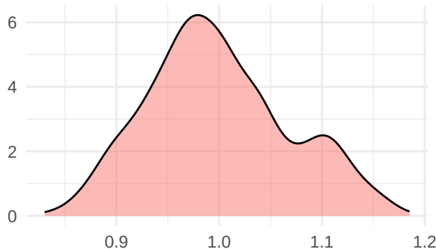
Posterior Density (Post-Warmup)
