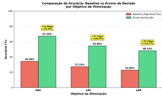
Figure 3: Accuracy Comparison: Baseline vs Decision Tree by Optimization Objective
