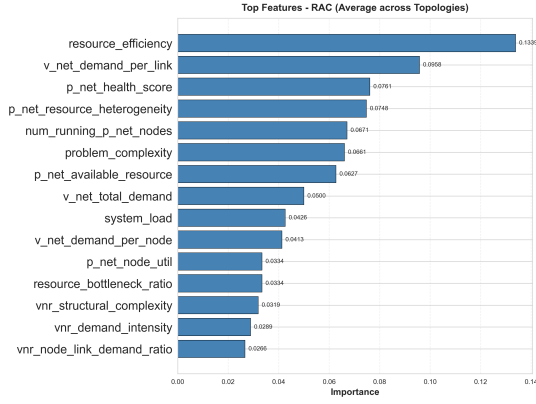
Figure 5: Feature Importance - RAC (Request Acceptance Rate). The top 15 most important features (average across topologies) for the RAC objective.
