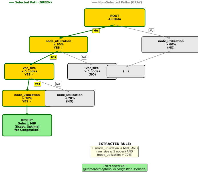
Figure 1: Example of decision path (root to leaf) in tree for VNE algorithm selection.
