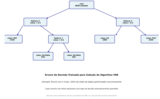
Fig. 8. Example of Decision Path in Tree
