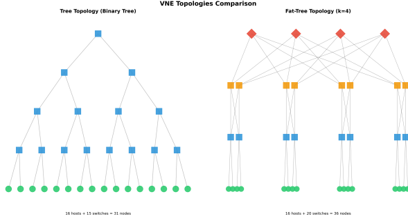
Fig. 3. Topology Comparison: Tree (Binary Hierarchical) and Fat-Tree (Datacenter). The Tree topology presents a traditional hierarchical structure with hosts at the base and switches at successive levels. The Fat-Tree presents a datacenter structure with k=4 , characterized by multiple paths and greater redundancy.
