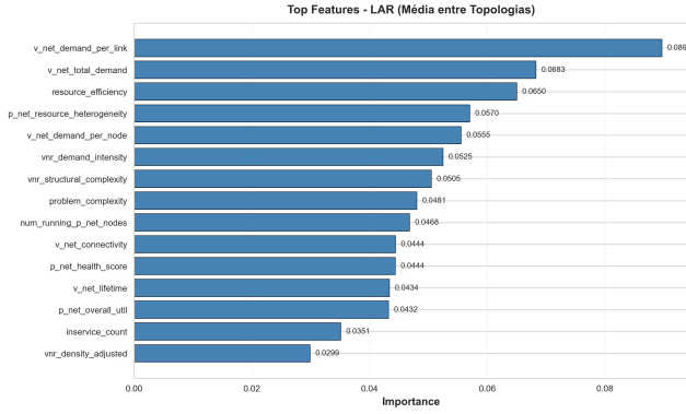
Fig. 11. Feature Importance - LAR (Long-Term Average Revenue). The top 15 most important features (average across topologies) for the LAR objective. VNR link demand ( v_net_demand_per_link ) is the most important feature with 0.090, followed by total demand ( v_net_total_demand ) with 0.068.
