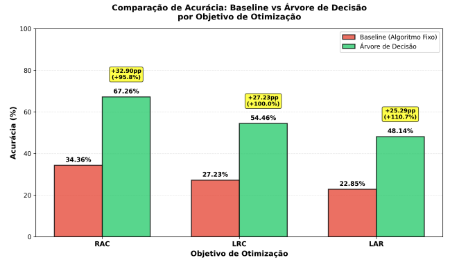
Fig. 6. Accuracy Comparison: Baseline vs Decision Tree by Optimization Objective
