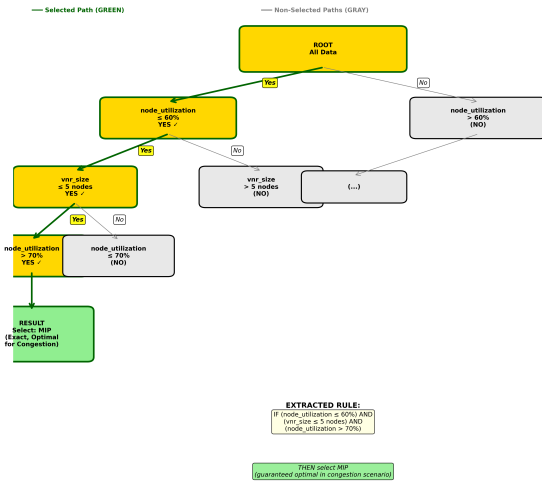
Fig. 2. Example of decision path (root to leaf) in tree for VNE algorithm selection.
