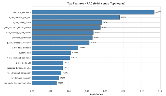
Fig. 9. Feature Importance - RAC (Request Acceptance Rate). The top 15 most important features (average across topologies) for the RAC objective. Resource efficiency ( resource_efficiency ) is the most critical feature with importance of 0.134, followed by VNR link demand ( v_net_demand_per_link ) with 0.096.
