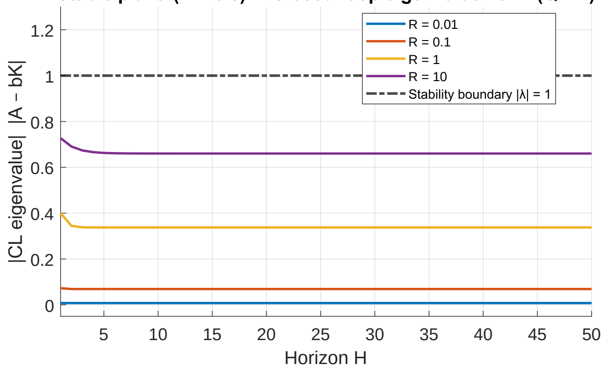
Stable plant ( A = 0.8 ) – Closed-loop eigenvalue vs H ( Q = 1 )
