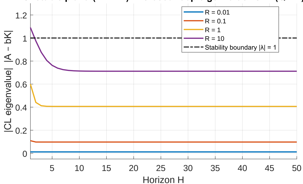
Unstable plant ( A = 1.2 ) - Closed-loop eigenvalue vs H ( Q = 1 )
