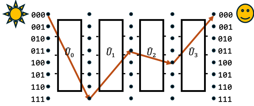
Figure 12: Analogy of information propagation on a quantum circuit with light transport.
