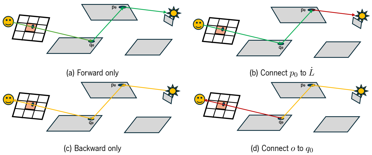
Figure 8: Different possibilities for sampling \{0, q_o, p_0, \dot{L}\} (besides figure 7)
