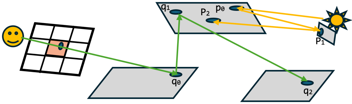
Figure 6: BiDirectional Path Tracing: forward and backward paths
