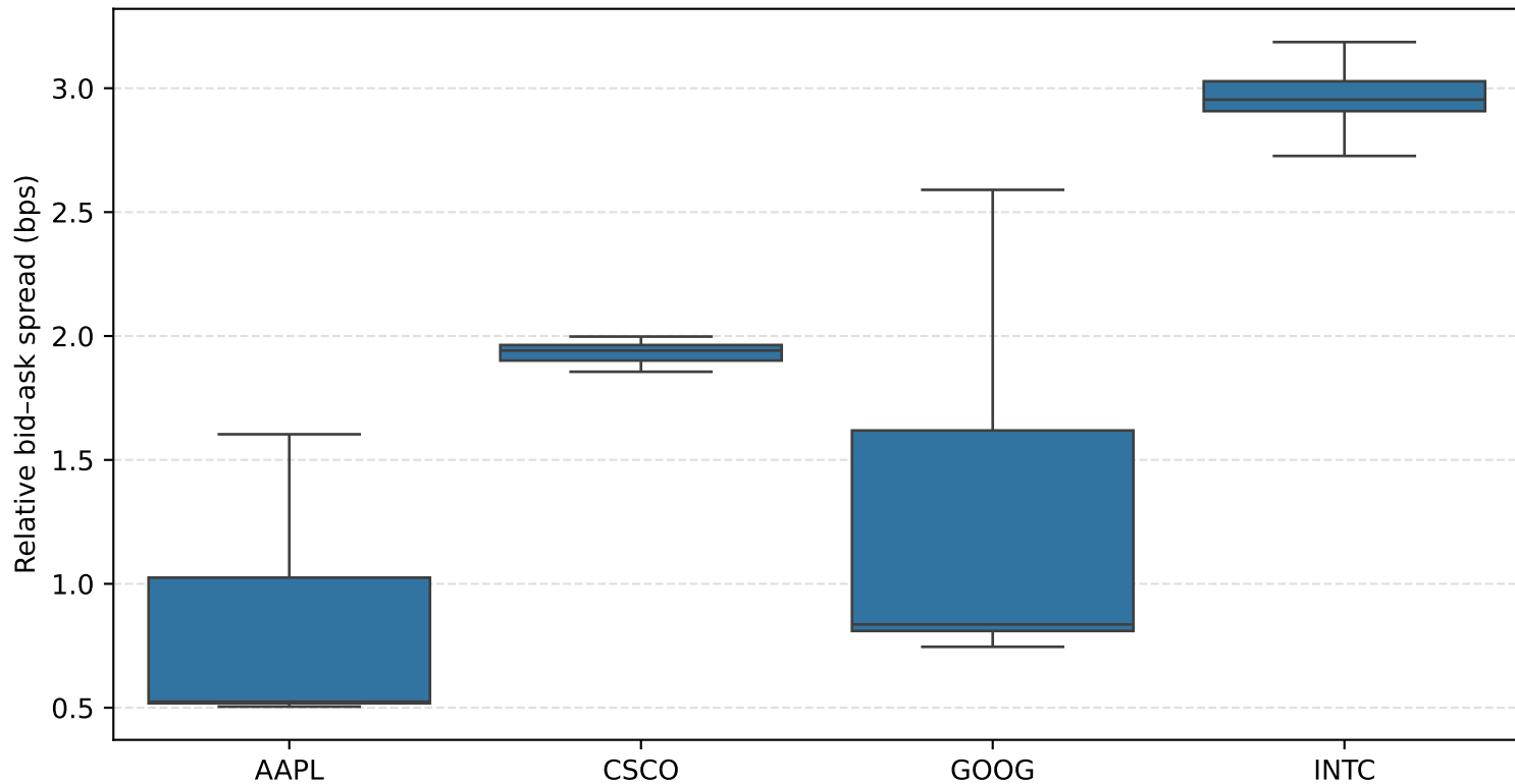
Distribution of relative bid-ask spreads across stocks
