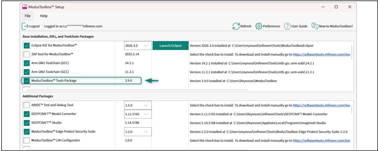
Figure 2 ModusToolbox™ version
