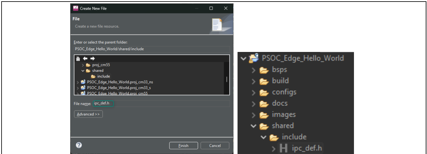
Figure 27 Create ipc_def.h
