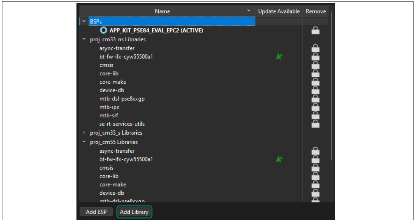
Figure 17 Add Library
