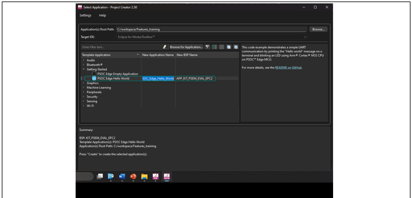
Figure 33 Selecting application
