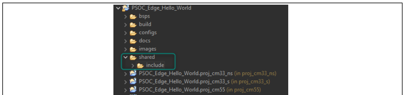
Figure 26 Shared folders
