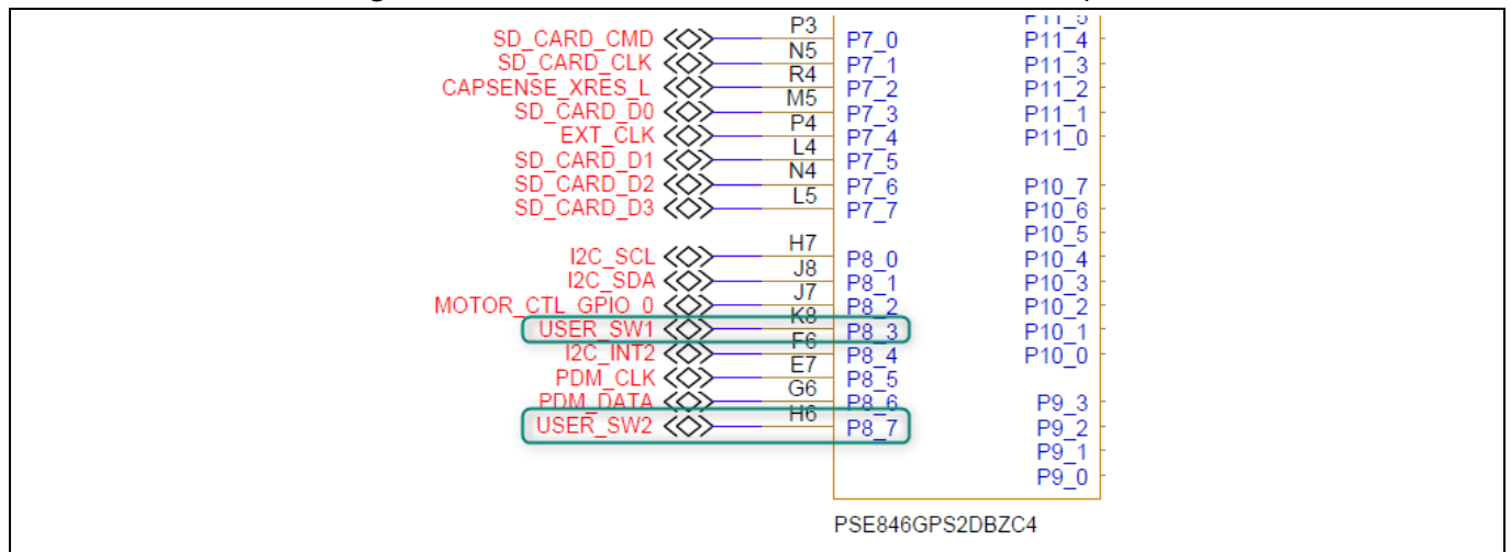
Figure 22 Connection of buttons in EVK schematics
