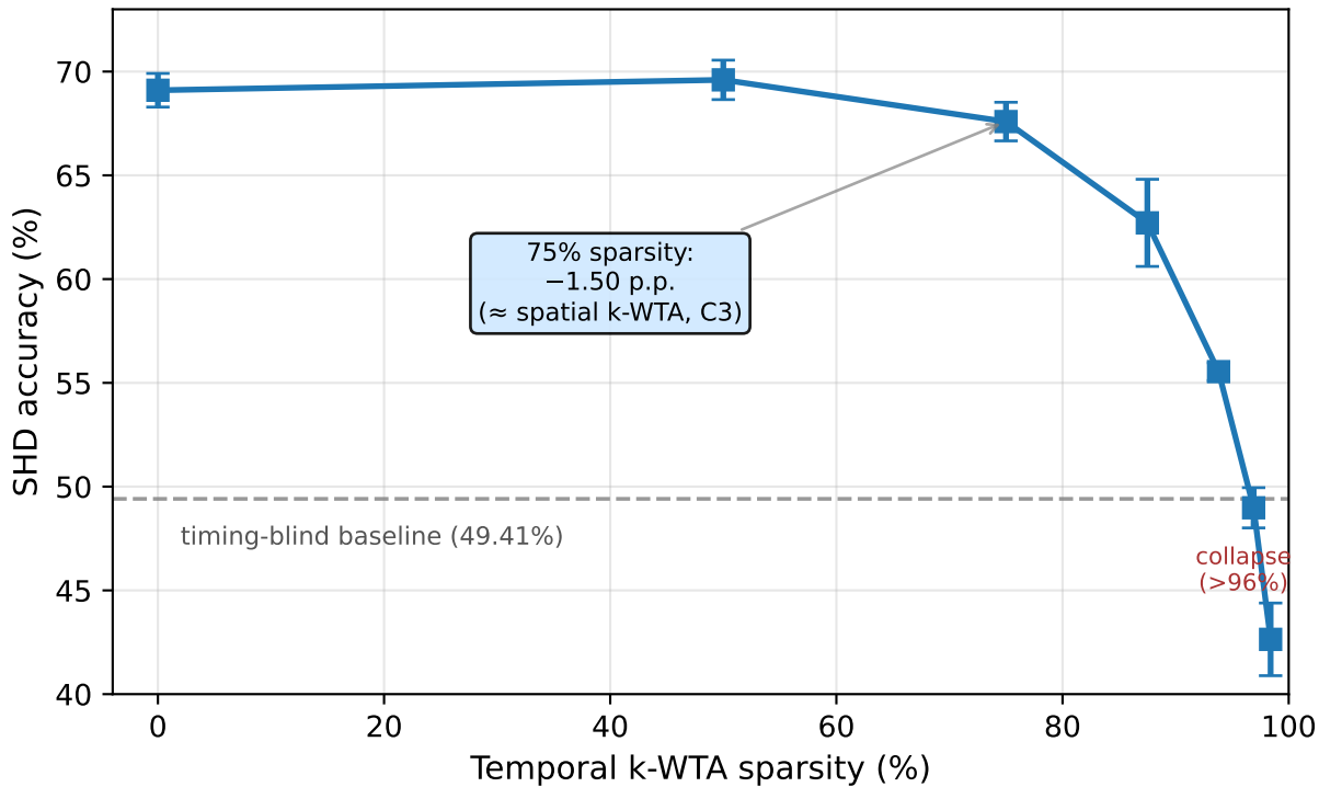
Temporal k-WTA: tolerant to 75%, collapses beyond 96%
