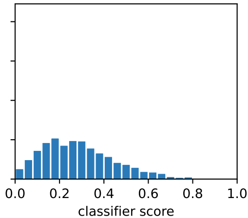
bins = 25
