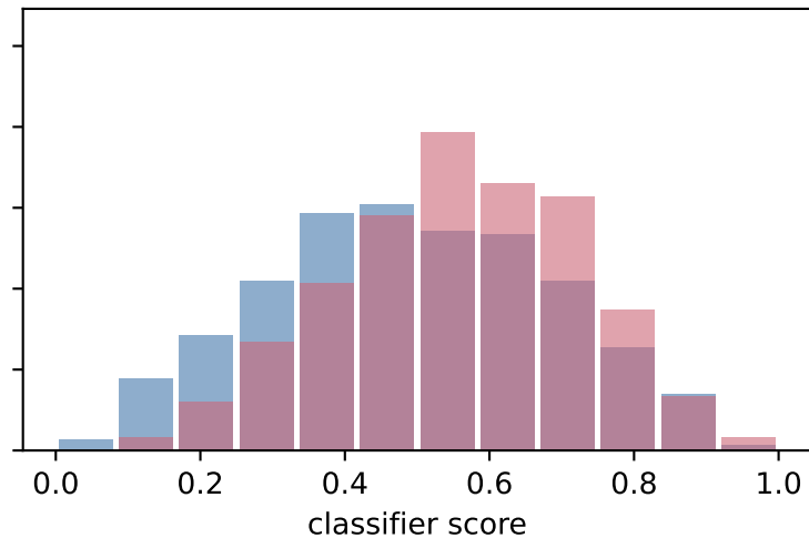
overlapping classes
