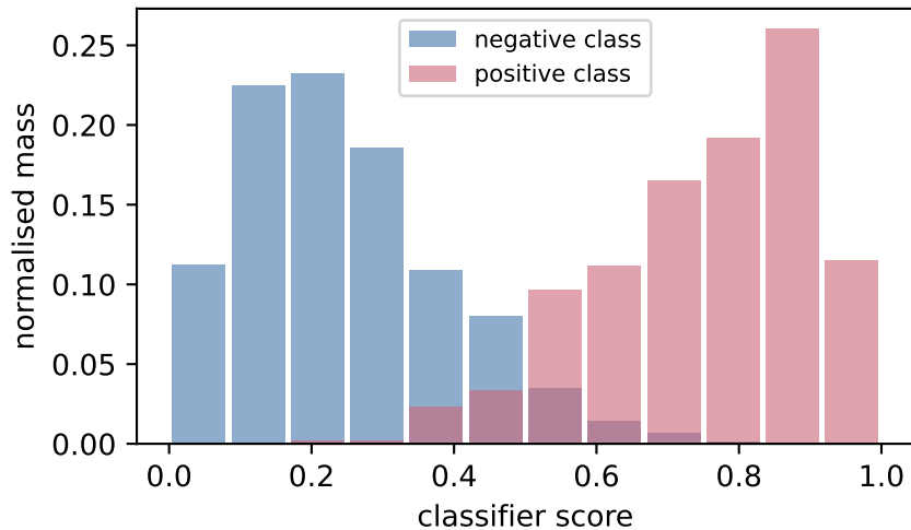
well-separated classes
