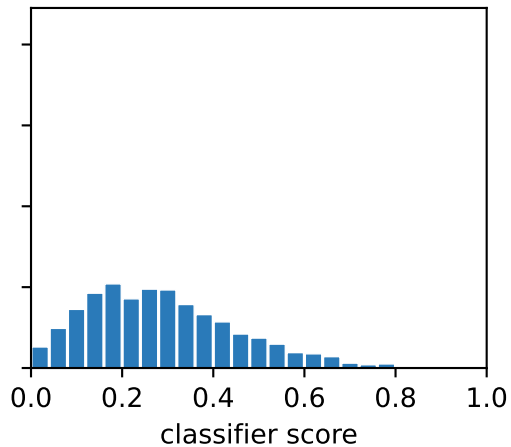
bins = 25
