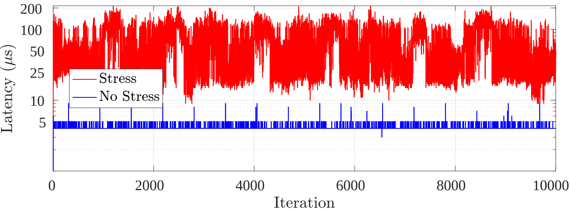
Latency for Scheduler: SCHED_DEADLINE n-19
