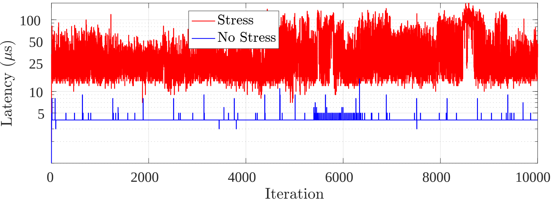
Latency for Scheduler: SCHED_FIFO n-19
