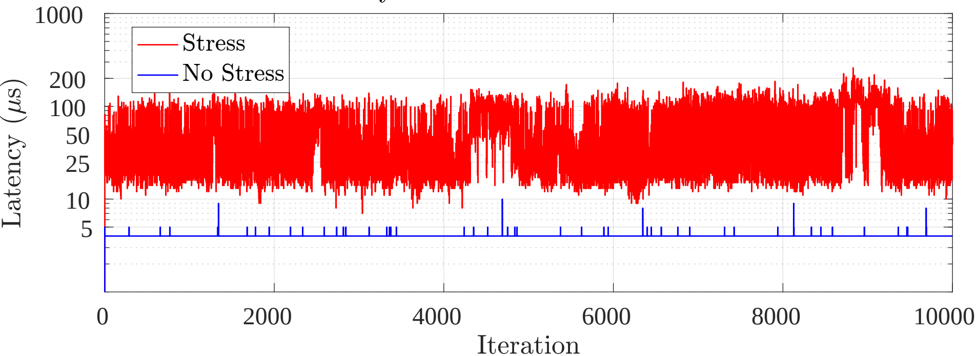
Latency for Scheduler: SCHED_RR n-19
