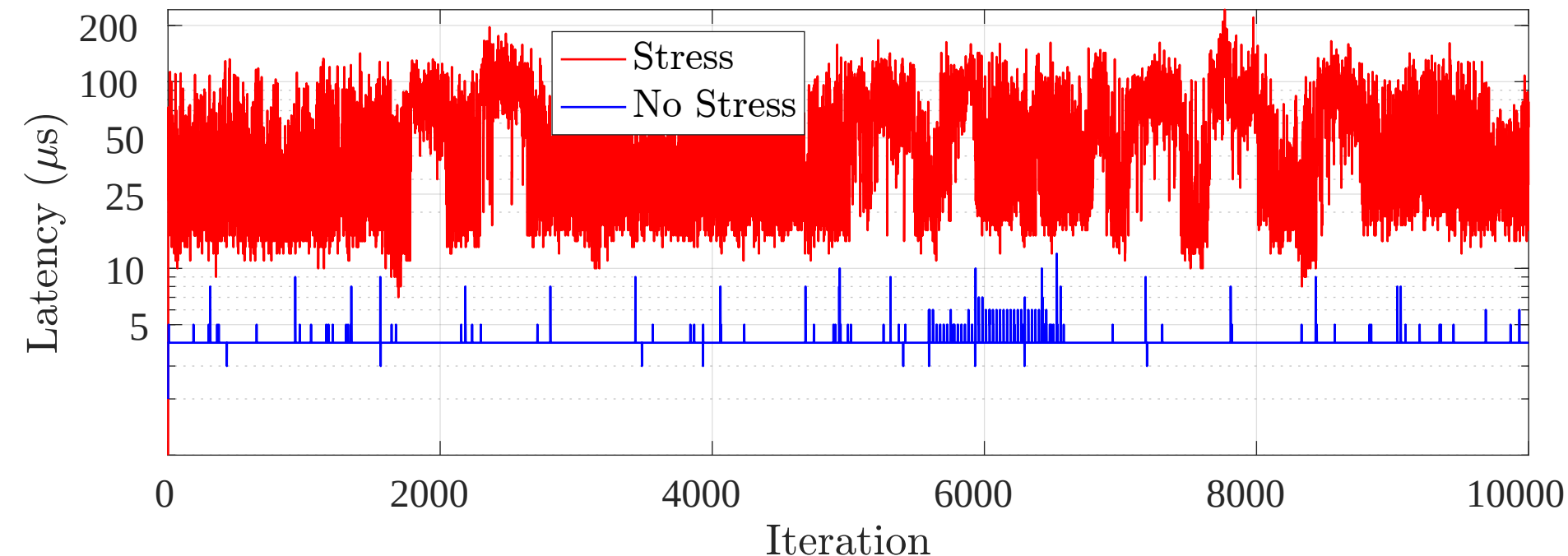
Latency for Scheduler: SCHED_RR n-19
