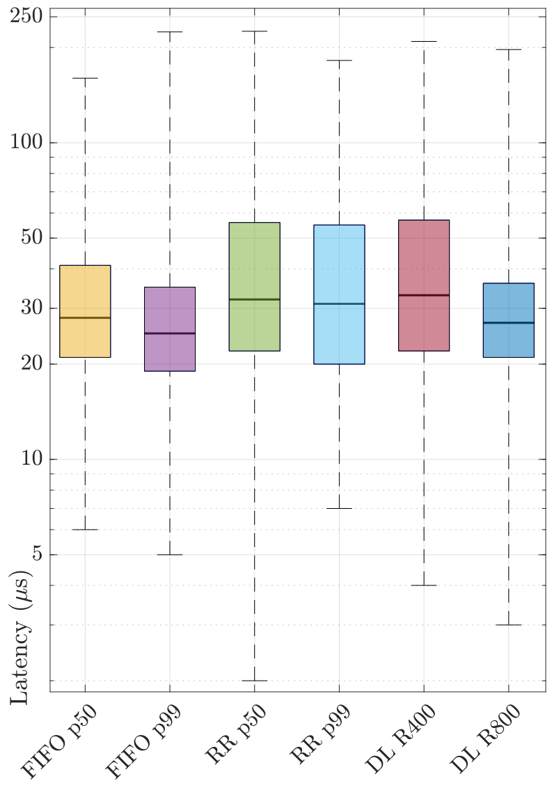
(b) PREEMPT_RT Kernel Under Stress
