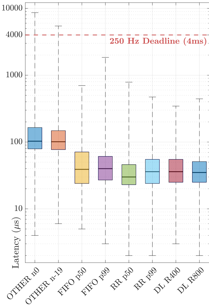
(a) Standard Kernel Under Stress
