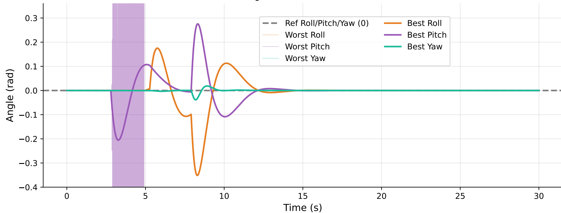
Attitude Tracking (Best vs Worst Case under Stress)
