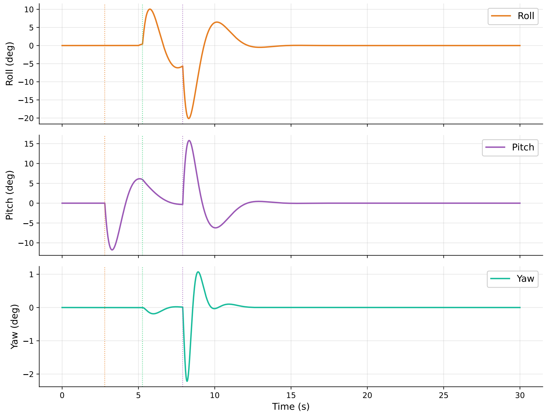
Kernel: preempt_rt | Policy: fifo_p50 | Load: idle — Attitude Response
