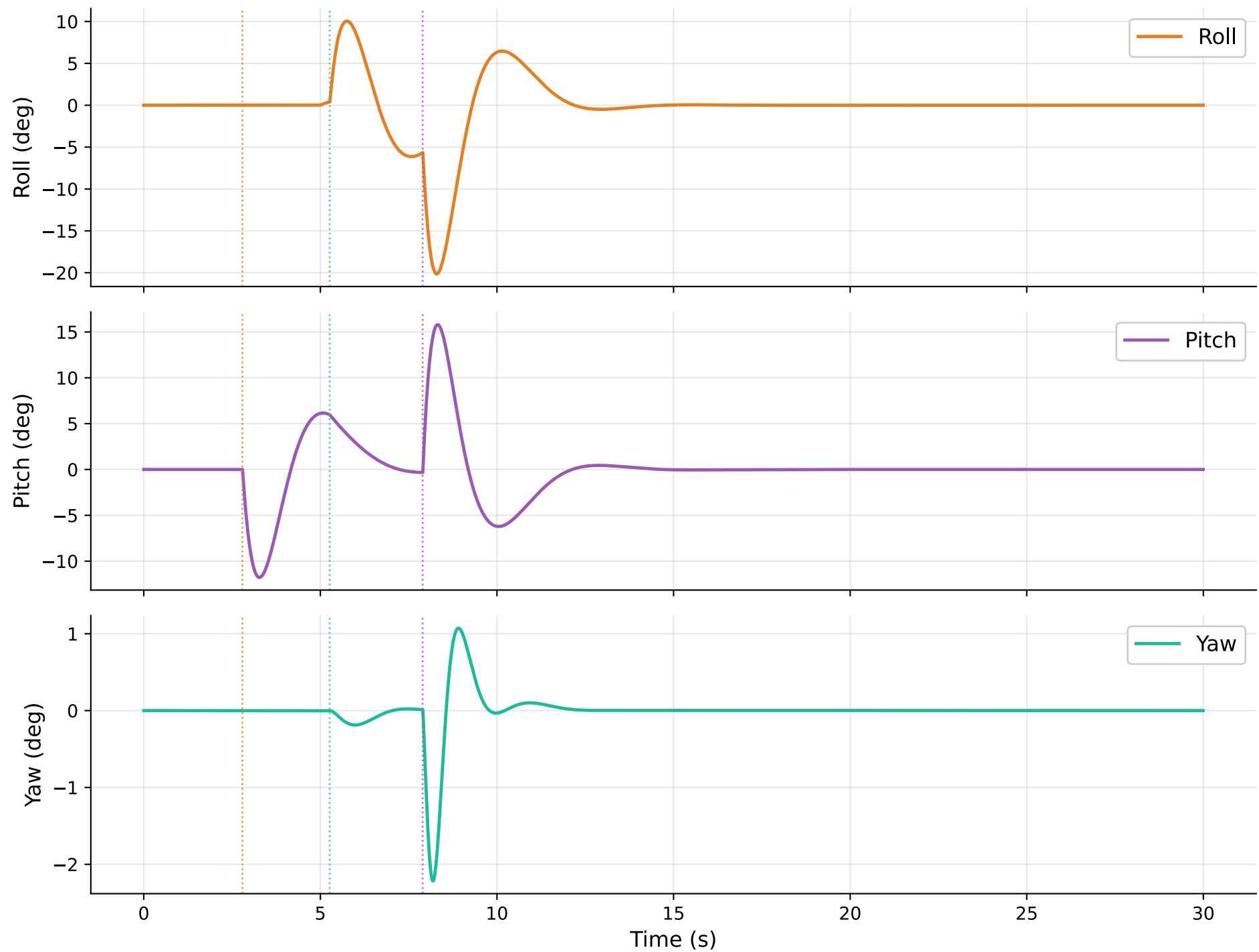
Kernel: preempt_rt | Policy: fifo_p99 | Load: idle — Attitude Response
