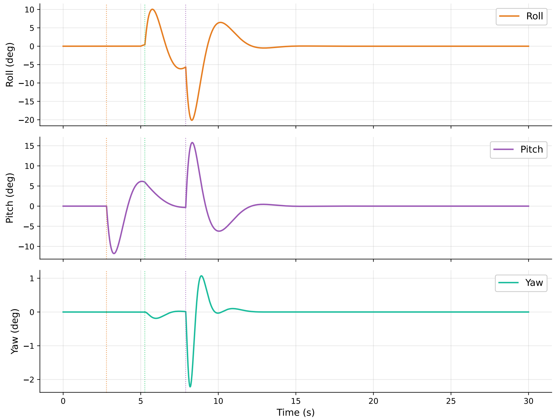
Kernel: preempt_rt | Policy: fifo_p99 | Load: stress — Attitude Response
