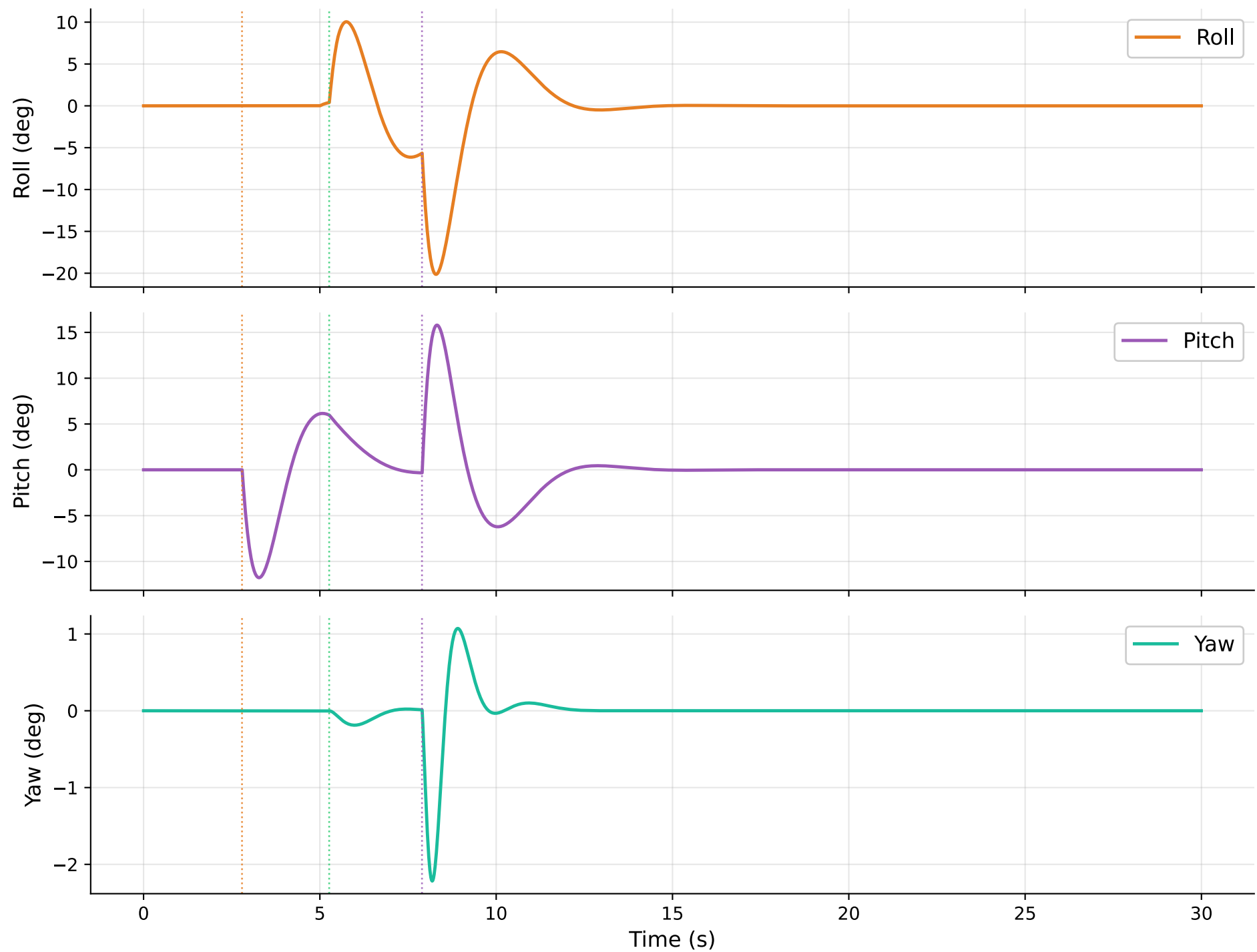
Kernel: preempt_rt | Policy: other_n0 | Load: idle — Attitude Response
