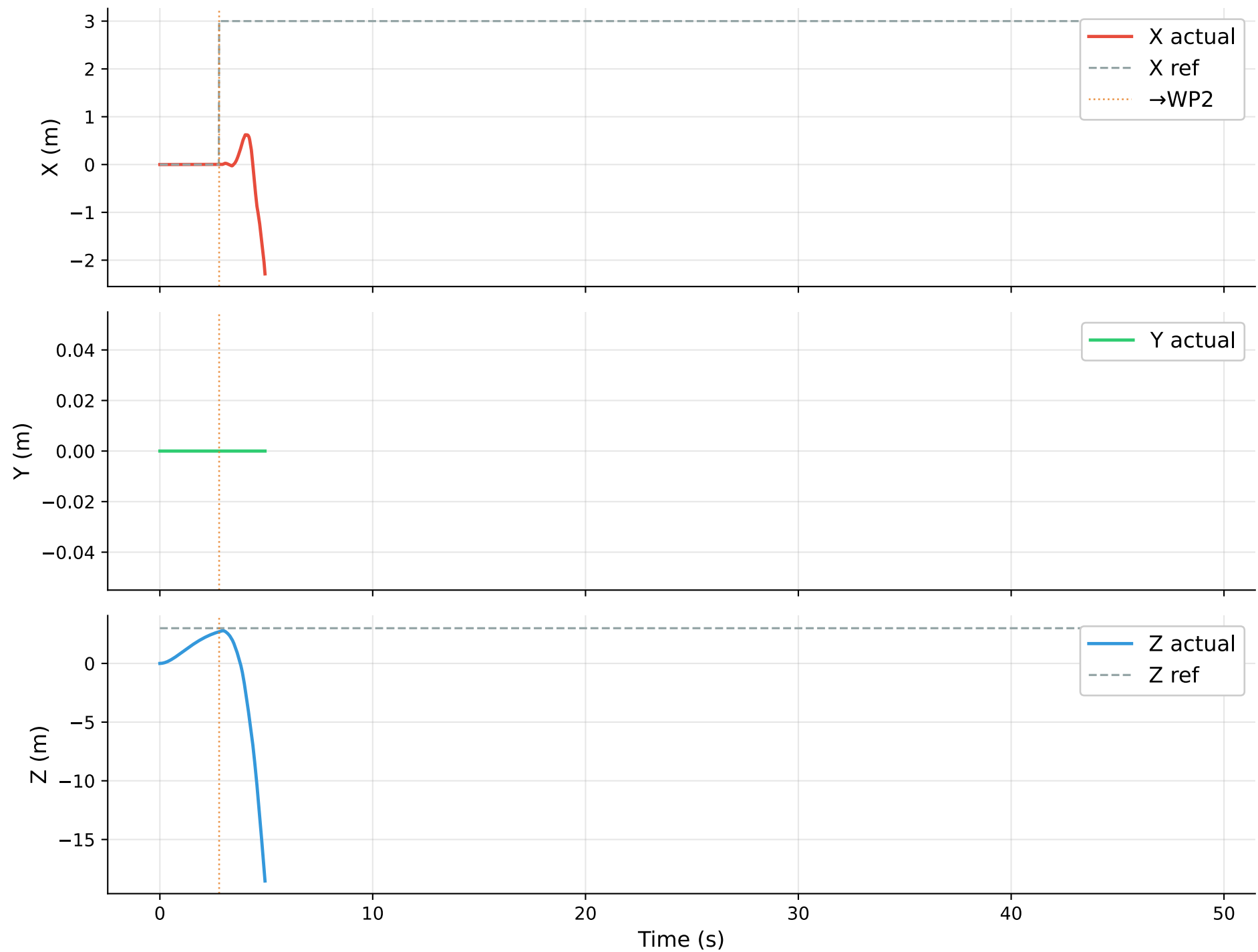
Kernel: preempt_rt | Policy: other_n0 | Load: stress — Position Response
