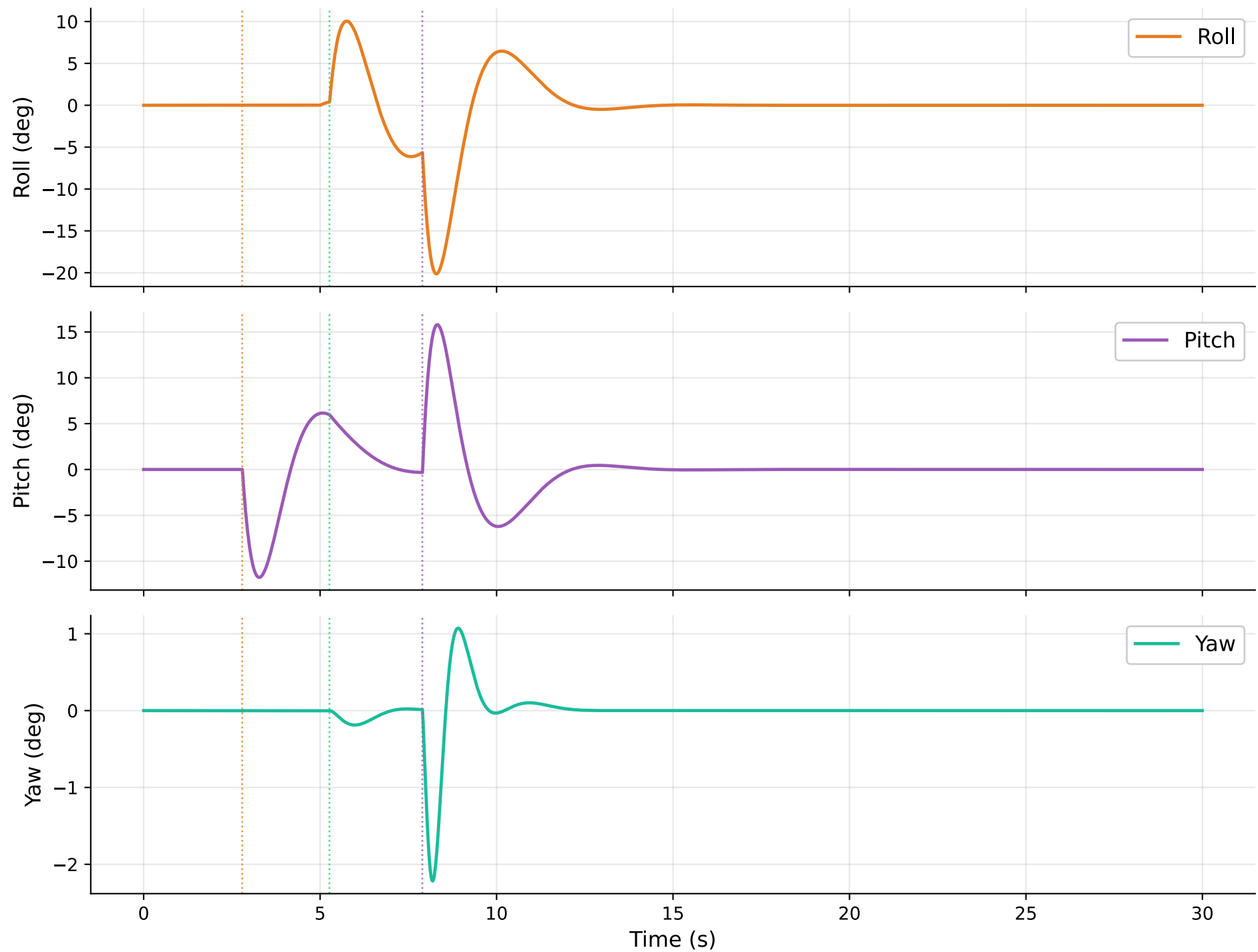
Kernel: preempt_rt | Policy: other_n19 | Load: idle — Attitude Response
