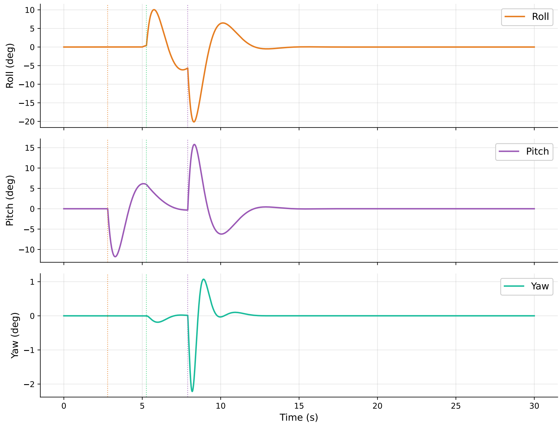
Kernel: preempt_rt | Policy: rr_p50 | Load: idle — Attitude Response
