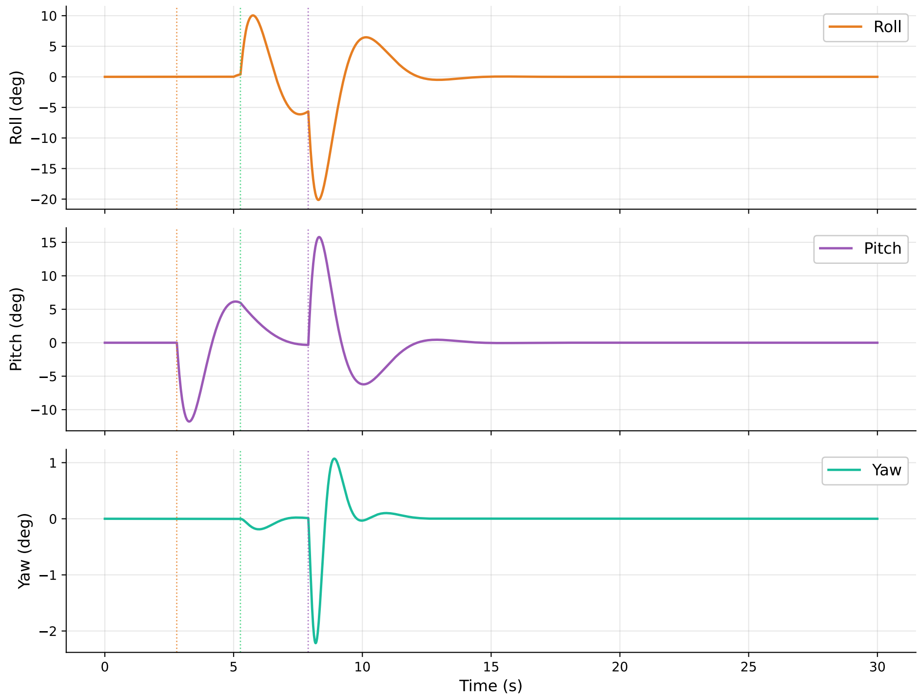
Kernel: preempt_rt | Policy: rr_p99 | Load: idle — Attitude Response
