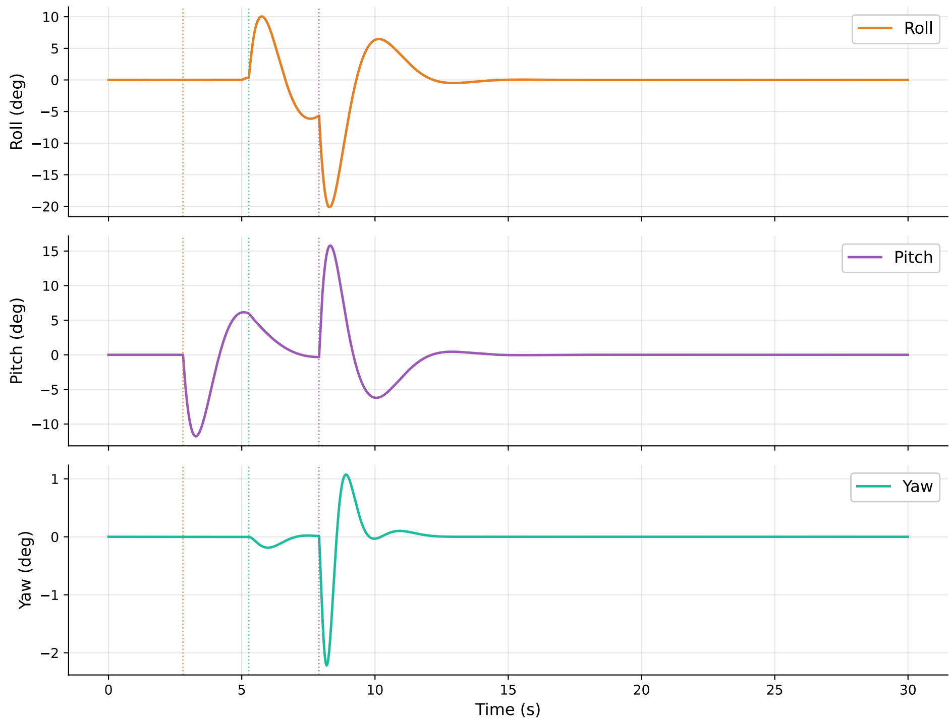
Kernel: preempt_rt | Policy: rr_p99 | Load: stress — Attitude Response
