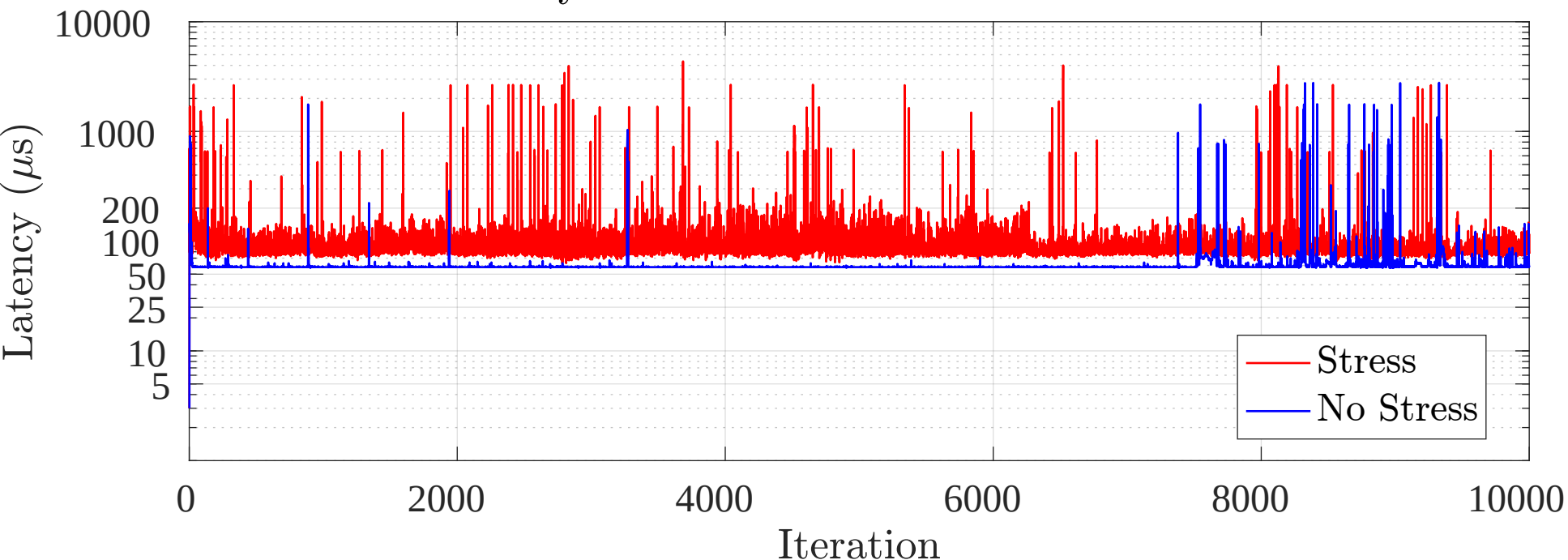
Latency for Scheduler: SCHED_OTHER n-19
