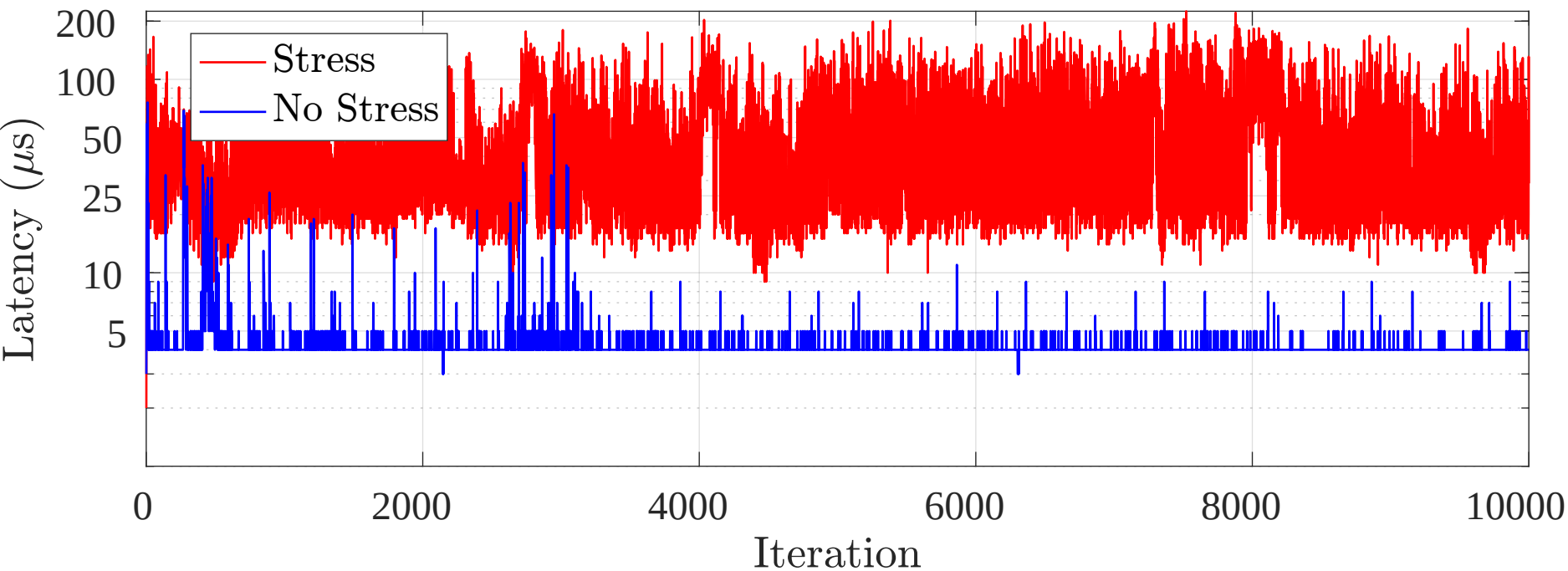
Latency for Scheduler: SCHED_RR p99
