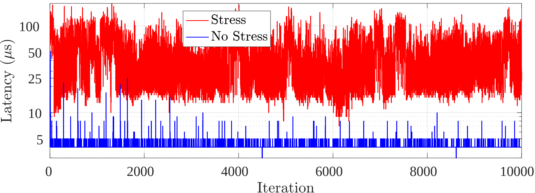
Latency for Scheduler: SCHED_RR p99
