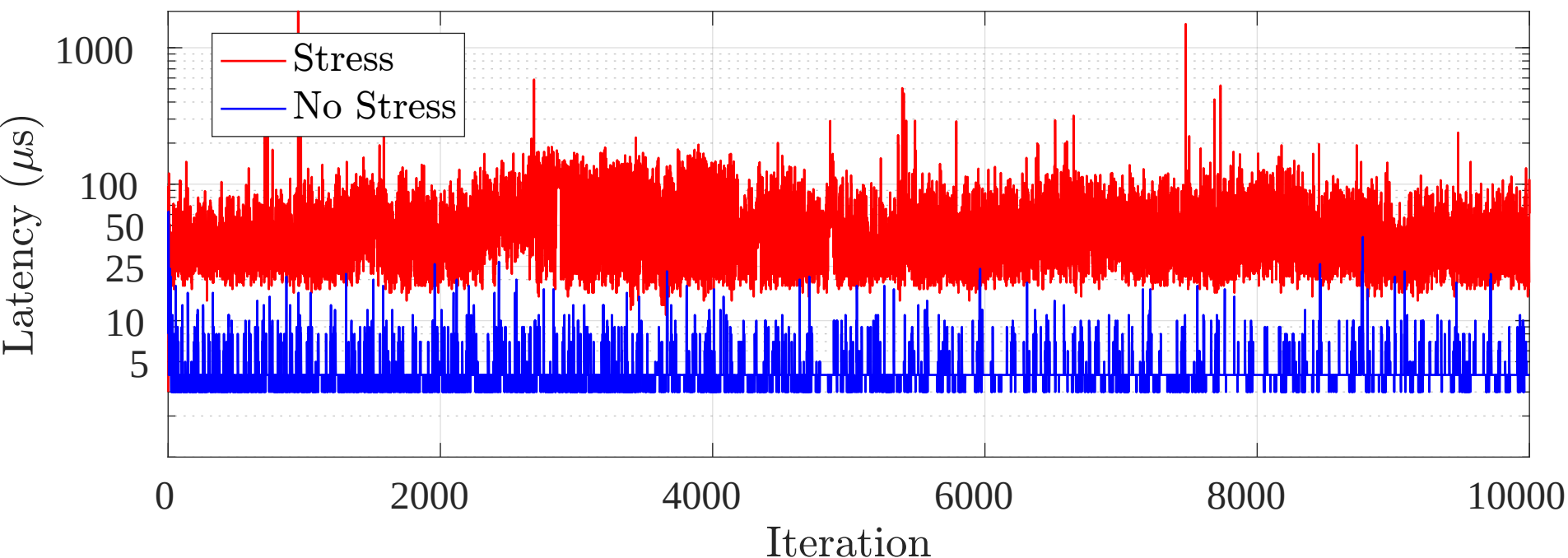
Latency for Scheduler: SCHED_FIFO p99
