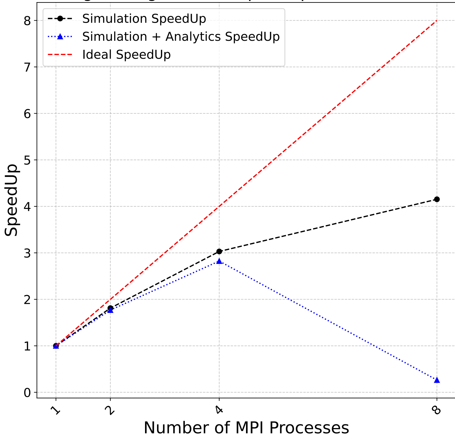
Strong Scaling (1node): SpeedUp vs MPI Processes
