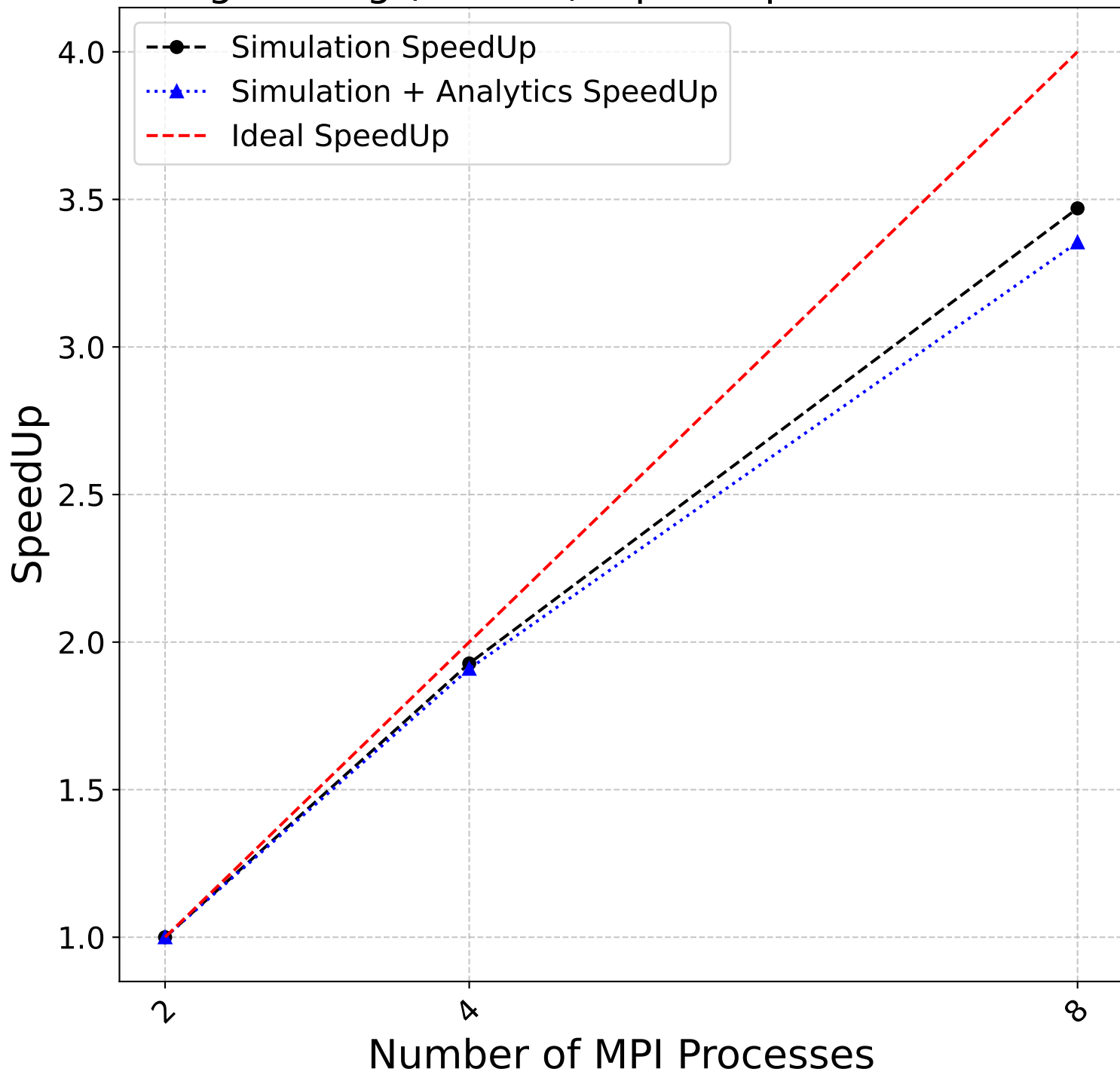
Strong Scaling (2nodes): SpeedUp vs MPI Processes
