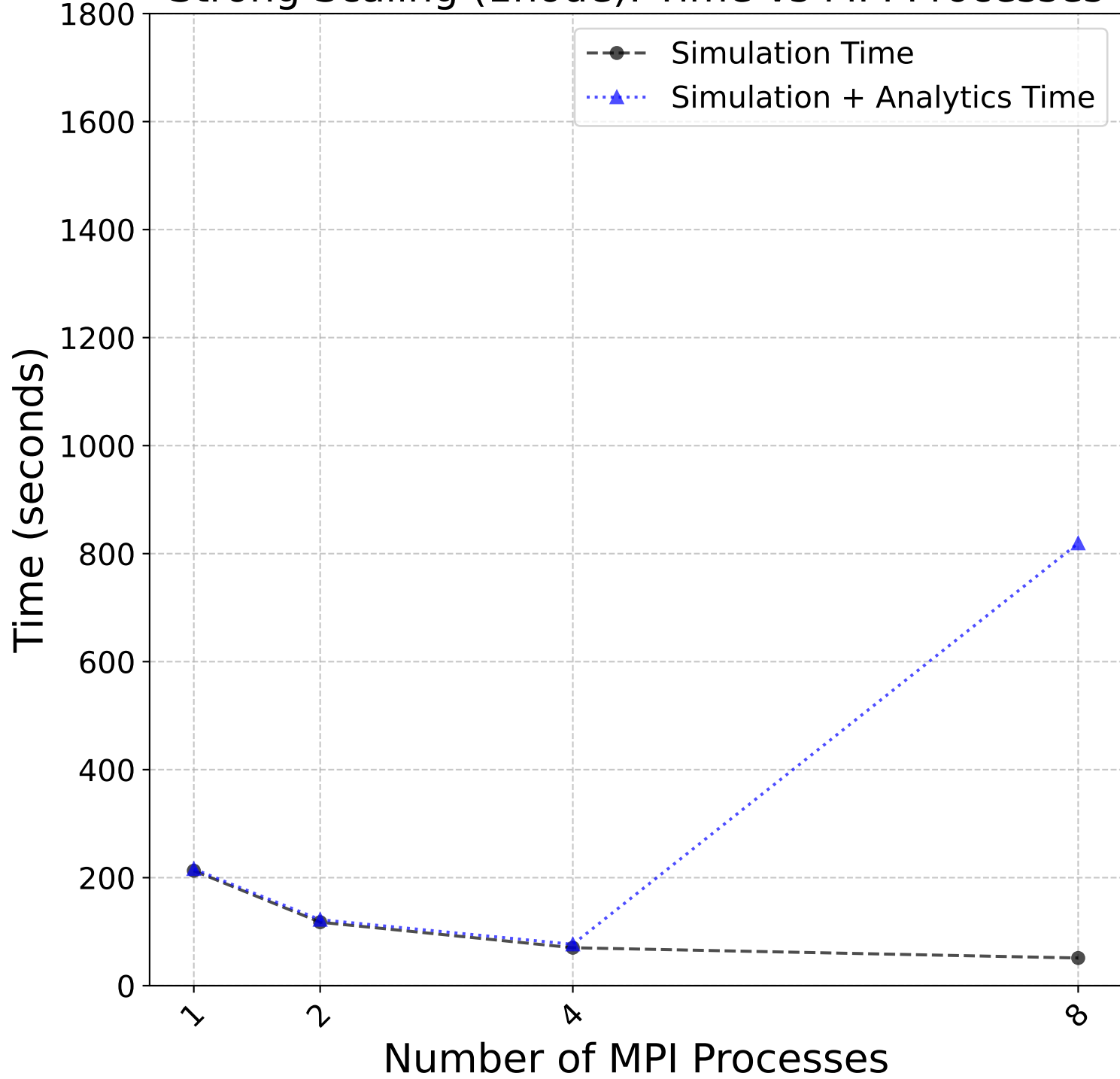
Strong Scaling (1node): Time vs MPI Processes
