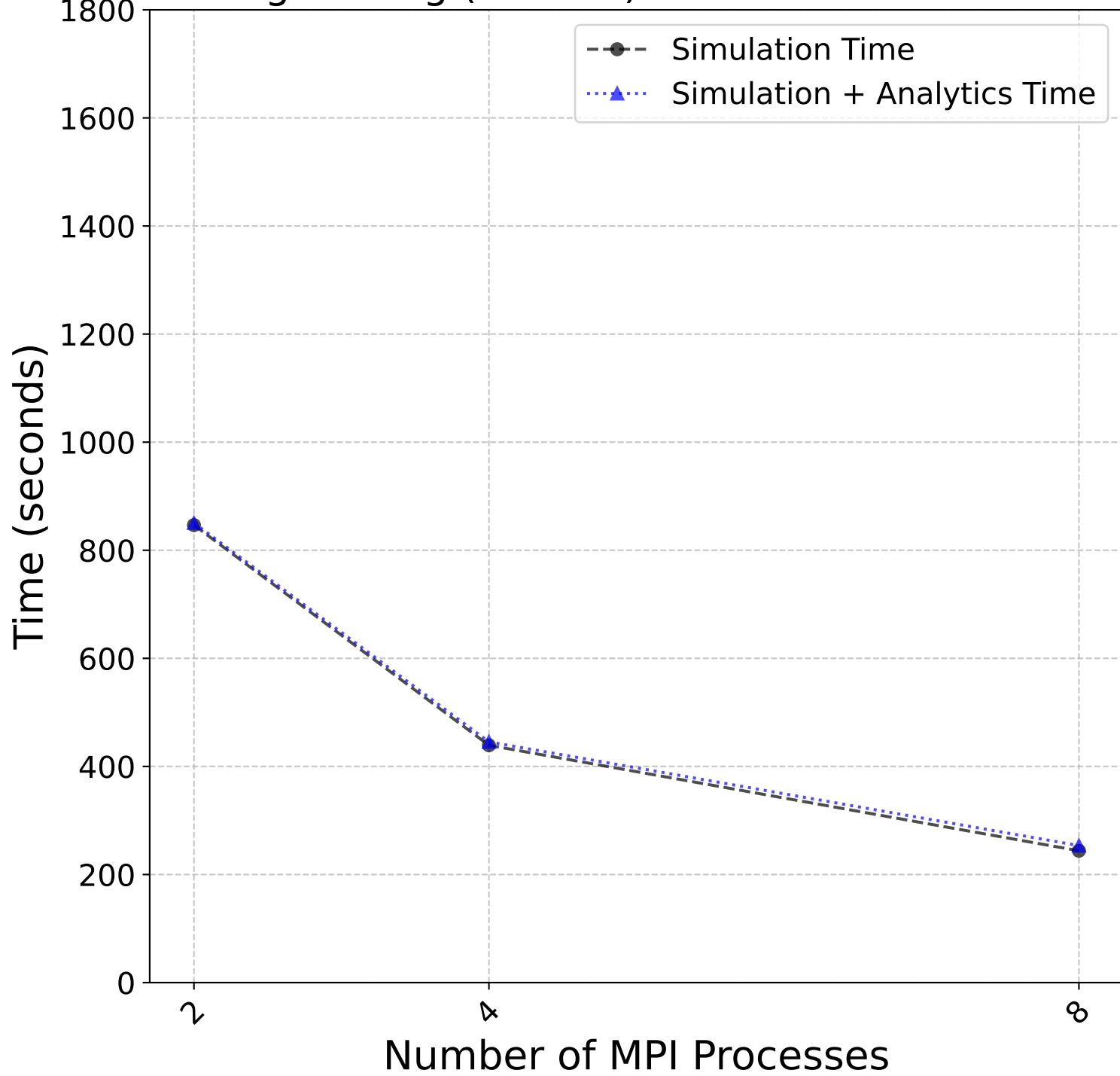
Strong Scaling (2nodes): Time vs MPI Processes
