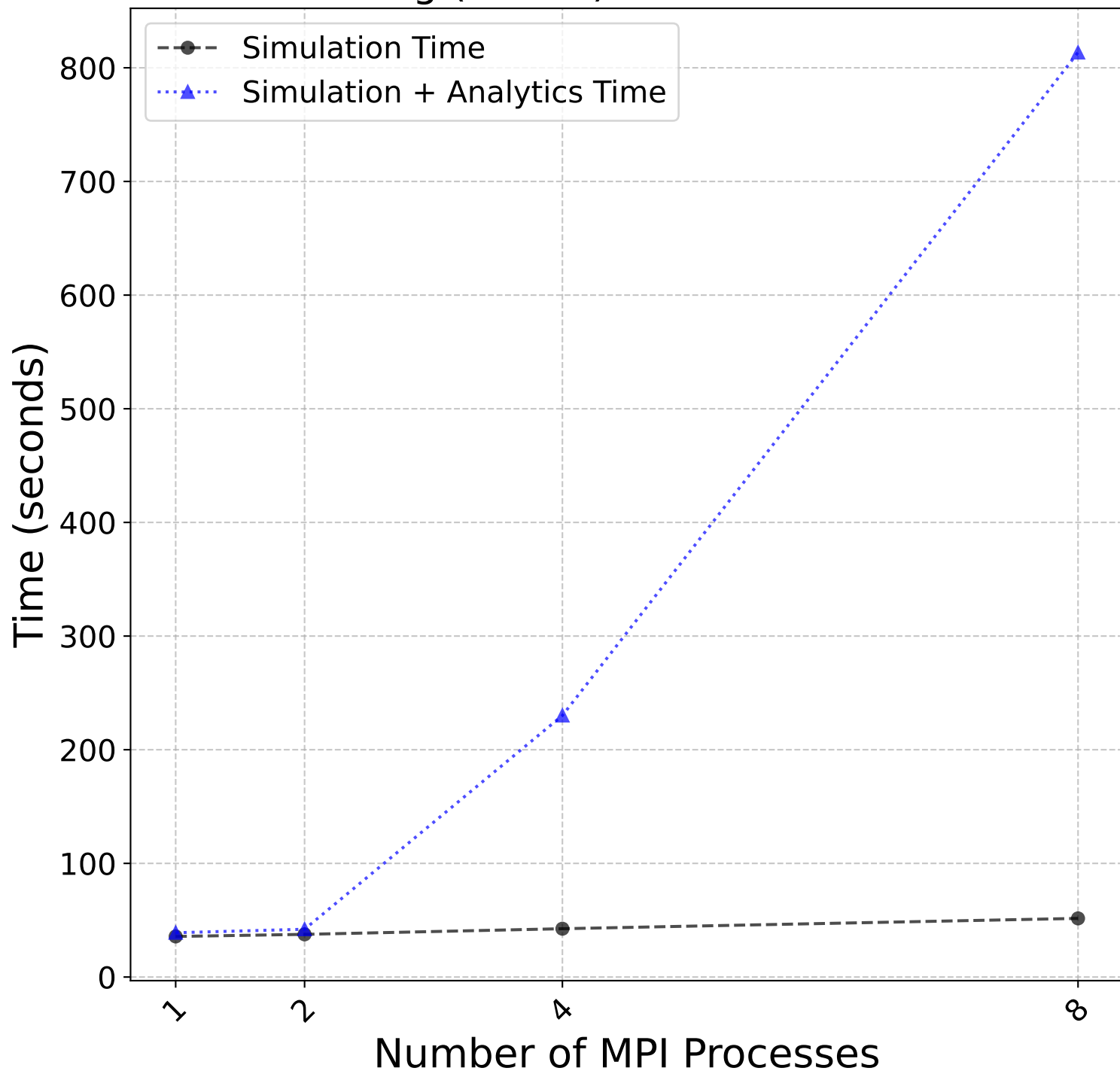
Weak Scaling (1node): Time vs MPI Processes
