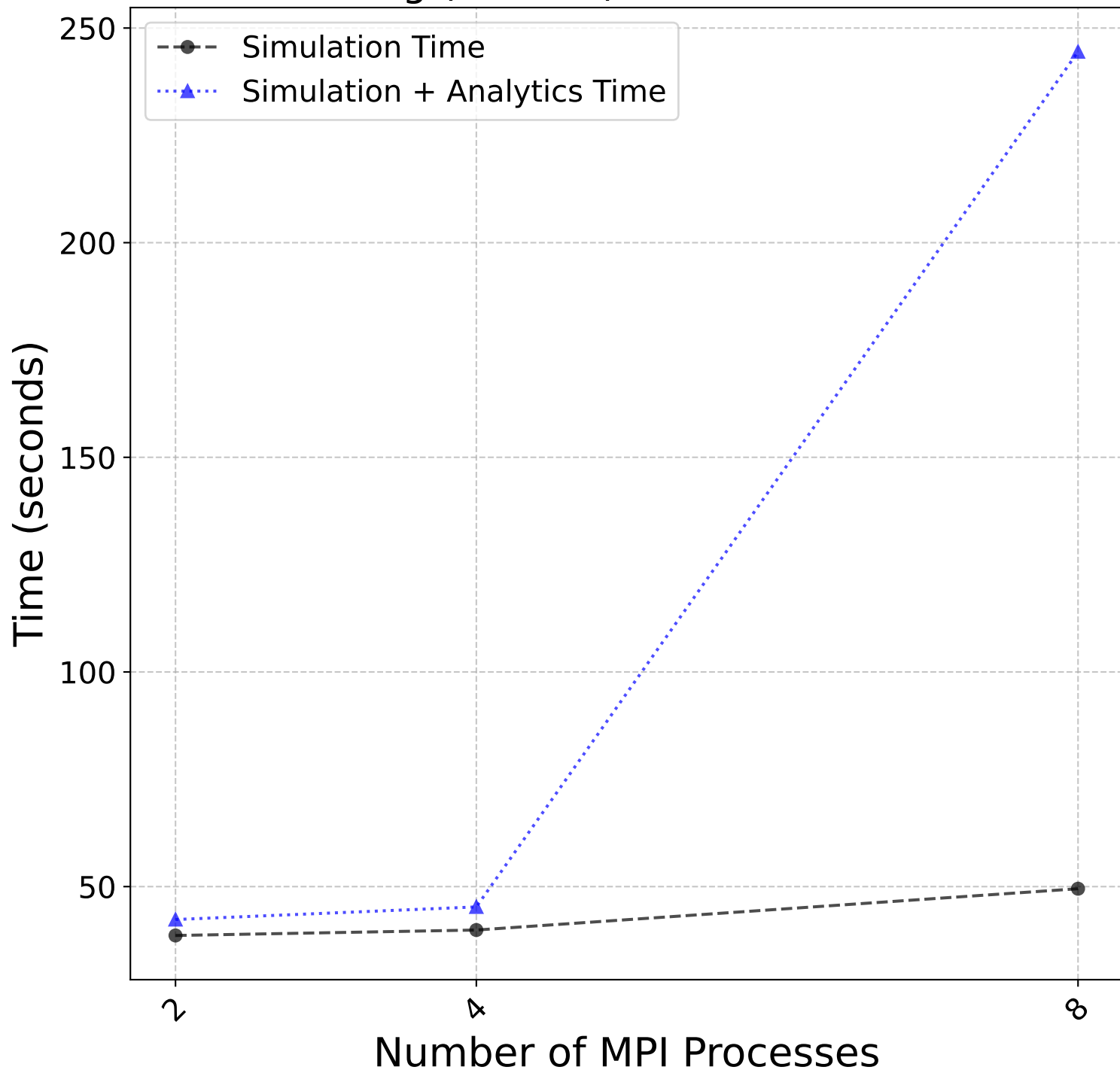
Weak Scaling (2nodes): Time vs MPI Processes
