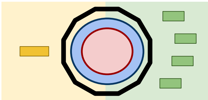
Scheduled process
