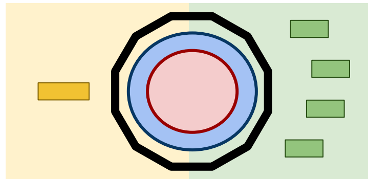
Event consumers
