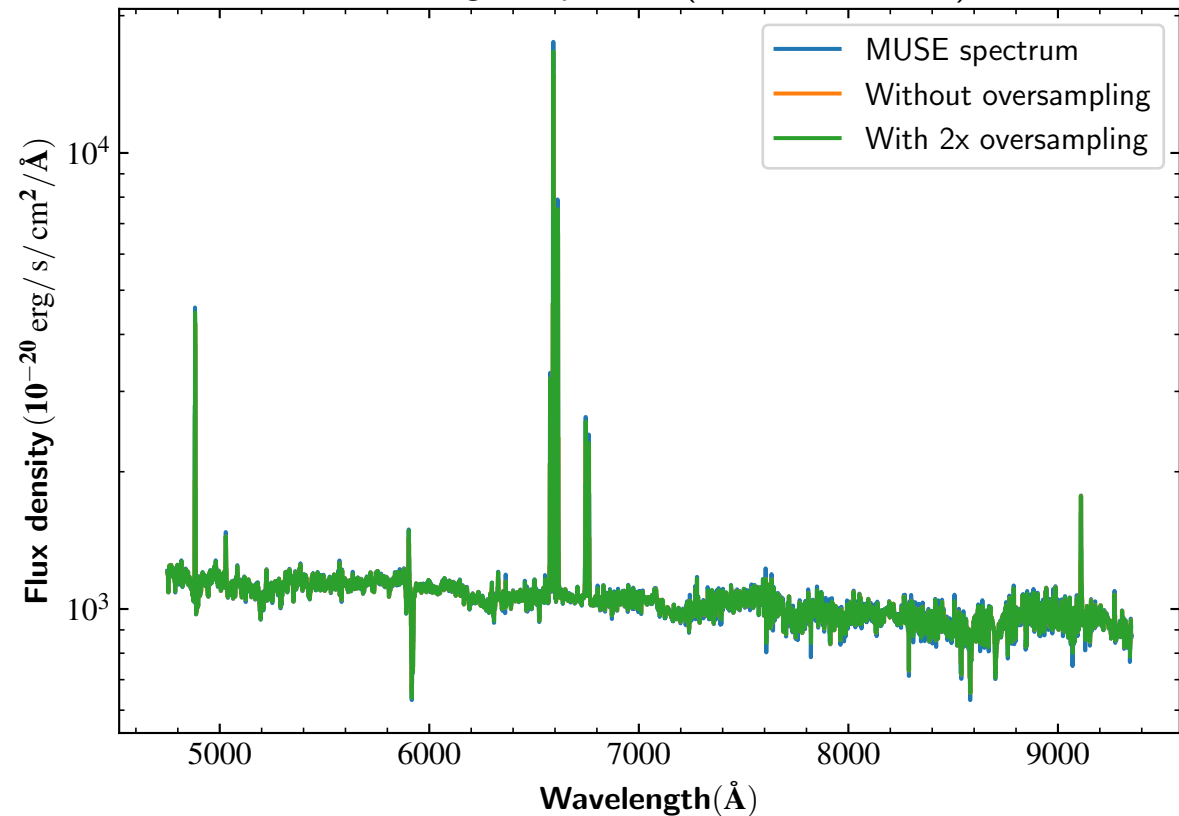
Rebinning comparison (flux conservative)
