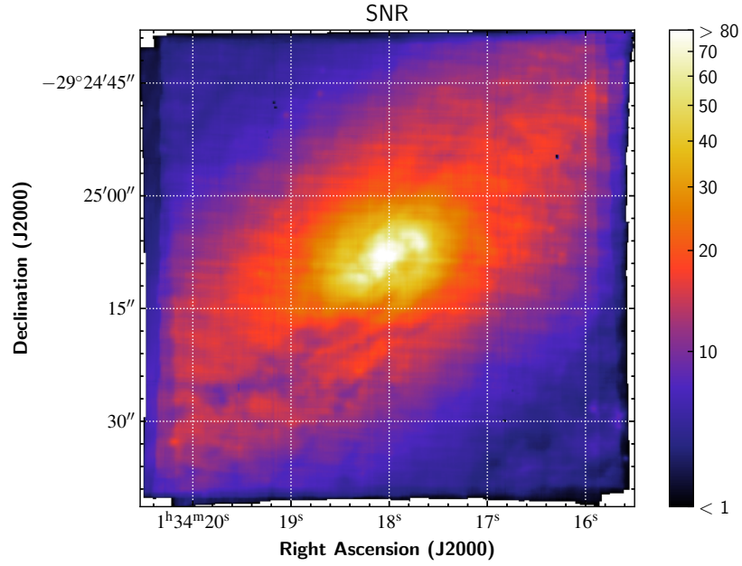
Figure 1: Signal-to-noise map of galaxy NGC 613. The observation was done with MUSE spectrograph. The image was enhanced (Gonzalez and Woods, 2018) by clipping the intensity range between 1 and 80. The image was colored by mapping the intensity of each pixel I(x, y) with a color scale using an arcsinh function (Lupton et al., 2004).
