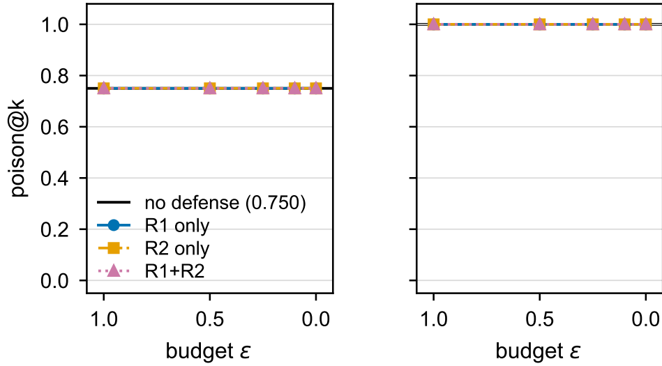
Figure 2: R1-constraint inertness. Adversarial-passage inclusion as a function of the constraint budget \epsilon , for the strictest ( \epsilon = 0 ) through the loosest ( \epsilon = 1 ) setting. Every constrained configuration coincides exactly with the unconstrained baseline – the lines are not merely close, the per-query values are identical – so the equivalence bound is \pm 0.0000 and the data exclude any effect on adversarial inclusion rather than an effect above some threshold.
