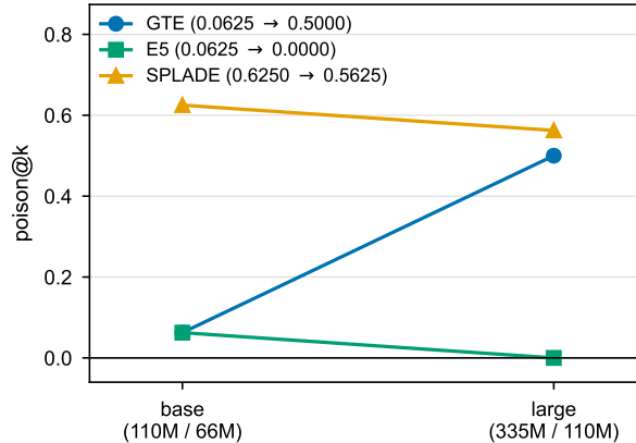
Figure 3: Text-attack susceptibility at base and large scale, within each encoder family and training recipe. GTE and E5 are equally resistant at base size and move in opposite directions when enlarged: E5 becomes fully resistant (0.0625 → 0.0000) while GTE becomes eight times more susceptible (0.0625 → 0.5000). The learned-sparse retriever is susceptible at both sizes. Since the only variable is the checkpoint, susceptibility is a per-checkpoint property that cannot be inferred from architecture, size or representation family.
