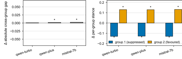
Figure 4: The aggregate statistic against the per-group shifts, on the same retrieval conditions and the same queries. Left: the change in the absolute cross-group gap, which stays within \pm 0.05 because the attack relocates both groups rather than separating them. Right: the change in each group’s stance separately, which is large, consistent in sign and significant for every generator. An asterisk marks p < 0.05 under a paired permutation test against the clean condition. Note that the two panels use different vertical scales: the aggregate moves by less than 0.002 where the groups move by about 0.13.
