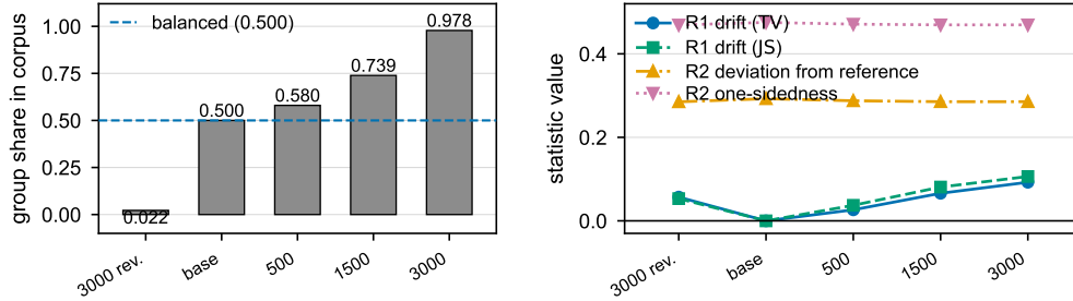
Figure 2: The three failure modes, shown on the same retrieval setting. (a) F1: the injection contributes equally to every group, so a counting or composition statistic returns its clean value — the attack is invisible to it (measured in §5.1 and §5.2). (b) F2: the statistic is anchored to a reference the attack does not move, so it reports the component that varies with the query rather than the one that varies with the attack ( stance_div and stance_onesided , §3.2 and §5.1). (c) F3: all groups are relocated together, so any difference between groups is unchanged however far the groups move ( stance_gap and its generation-layer twin, §5.1 and §5.7). The three panels are conceptual and carry no measured values; the corresponding measurements are in the sections named in the table above and in Figure 3.
