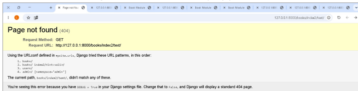
Figure 9: index2/text/ does not match <int:val1> — 404 Not Found
