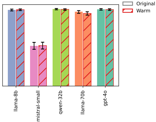
AdvBench
